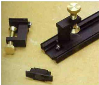
The bespoke clamps slide into the underside of the extrusion
