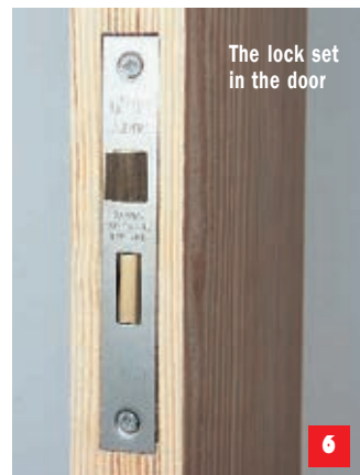
A completed mortise and face plate cut. The corners were squared with the corner chisel
