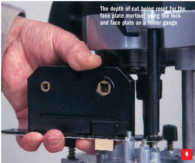
The mortise being cut with a 'drilling' action
