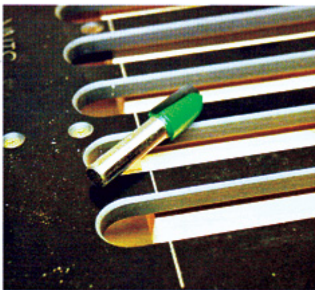
▲ The jig comes supplied with the correct cutter as well as a 30mm guide bush
