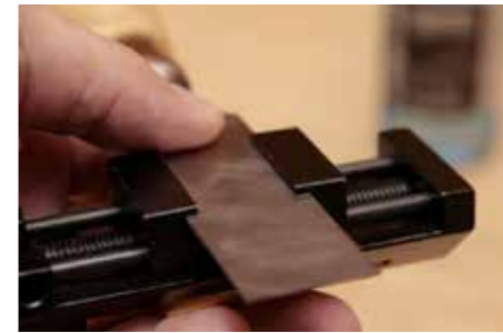
▲ As the guide is tightened, the blade is lifted until it is secured against the side tabs
