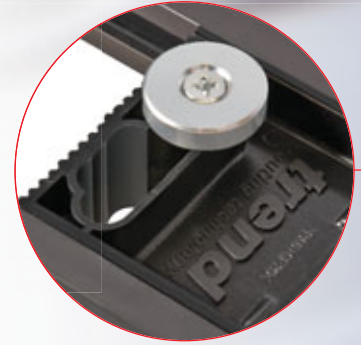
Adjustable stops plus three preset stop positions for 20mm, 25mm & 30mm hinge leaf.
