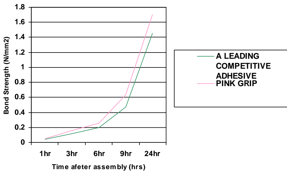
Early Adhesive bond Strength (wood/wood)
