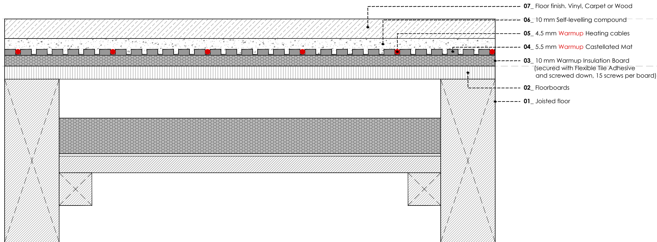
WARMUP CASTELLATED MAT SYSTEM. TIMBER SUBFLOOR AND VINYL, CARPET OR WOOD (with Warmup insulation boards)
