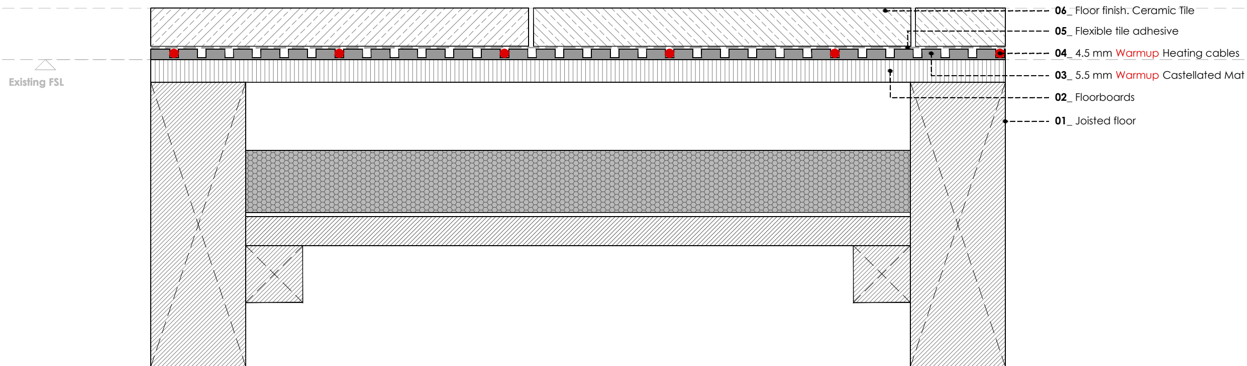
WARMUP CASTELLATED MAT SYSTEM. TIMBER SUBFLOOR AND TILES
