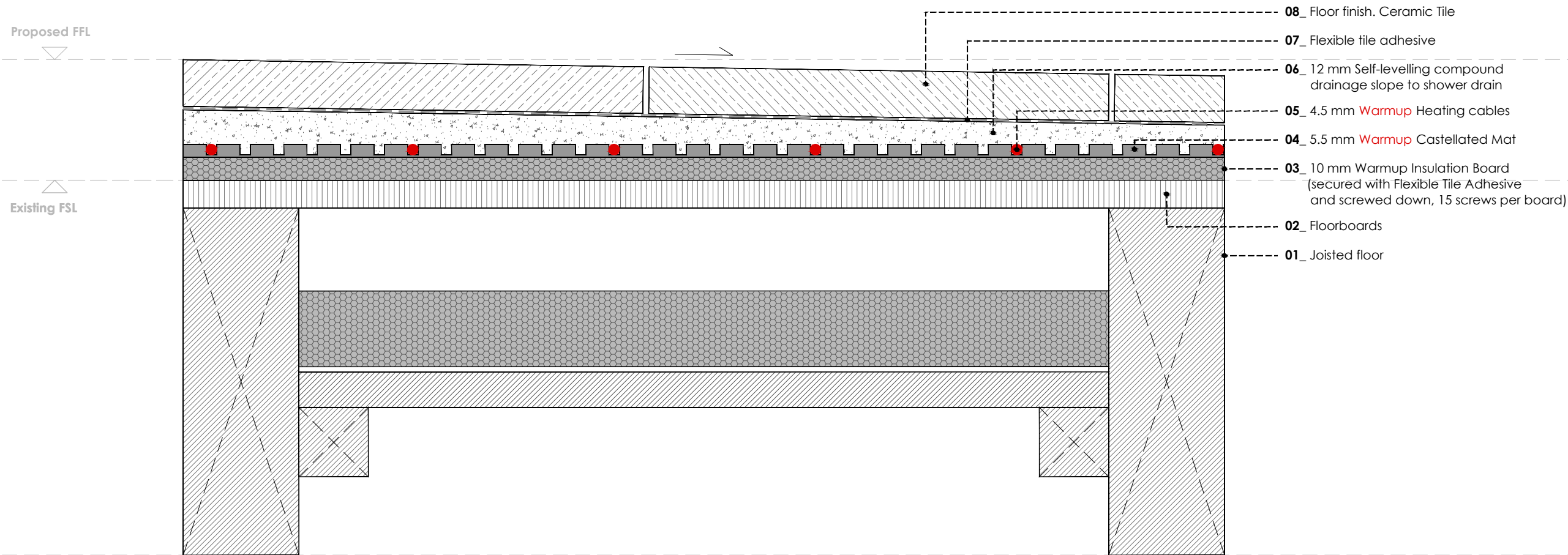
WARMUP CASTELLATED MAT SYSTEM. TIMBER SUBFLOOR WITH DRAINAGE SLOPE FOR WETROOMS (with Warmup insulation boards)
