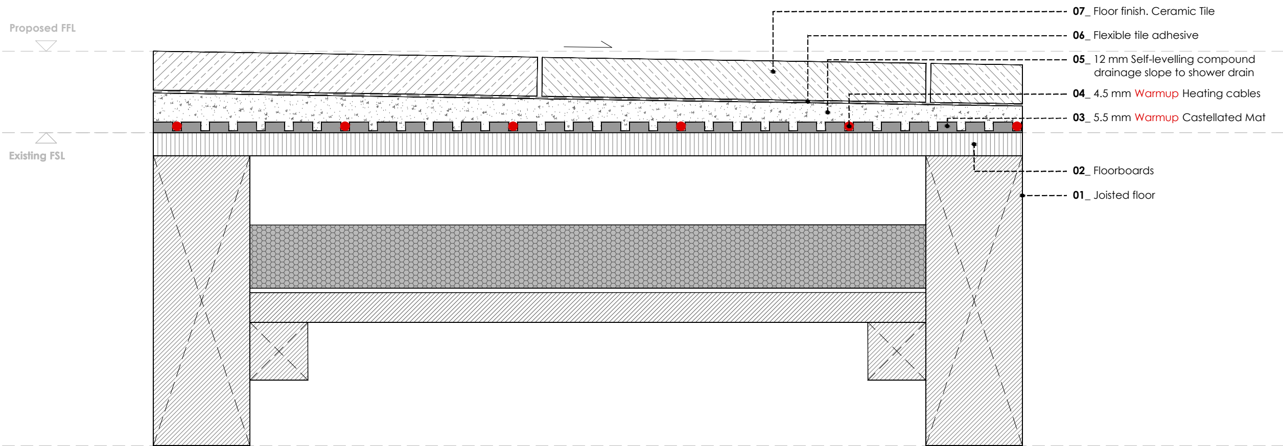
WARMUP CASTELLATED MAT SYSTEM. TIMBER SUBFLOOR WITH DRAINAGE SLOPE FOR WETROOMS
