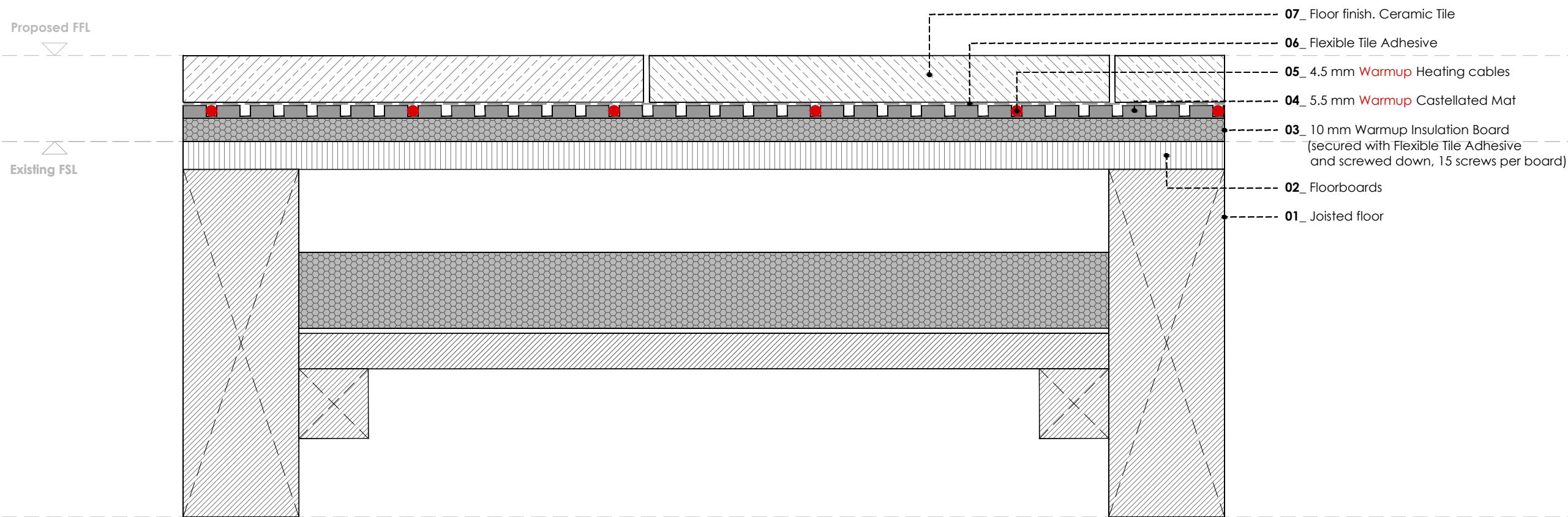
WARMUP CASTELLATED MAT SYSTEM. TIMBER SUBFLOOR AND TILES (with Warmup insulation boards)
