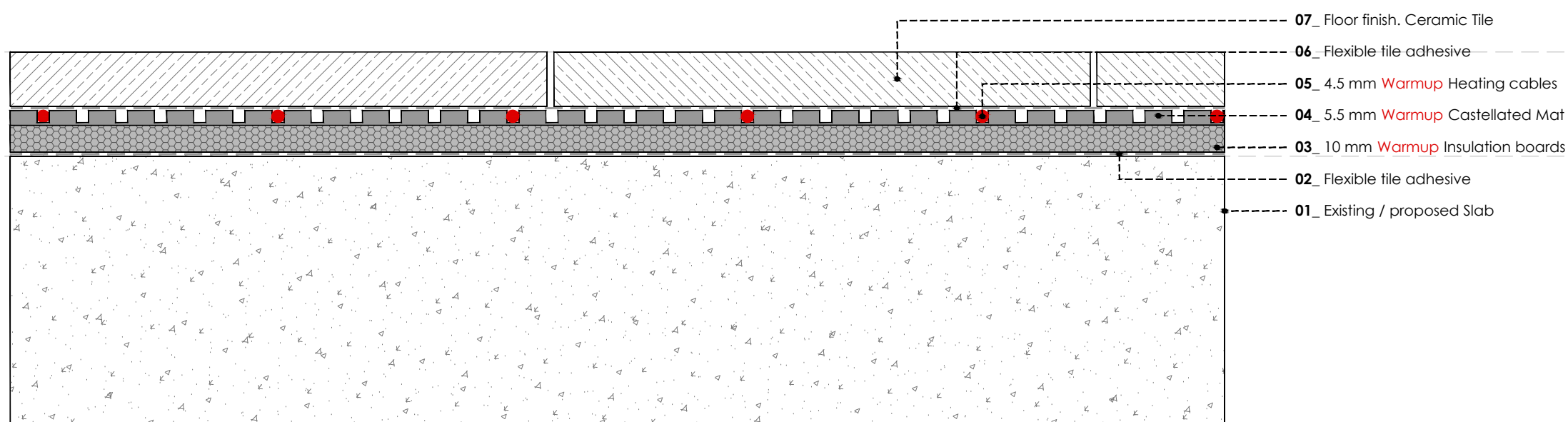
WARMUP CASTELLATED MAT SYSTEM. CONCRETE SUBFLOOR AND TILES (with Warmup insulation boards)
