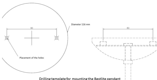
Drilling template for mounting the Bestlite pendant
